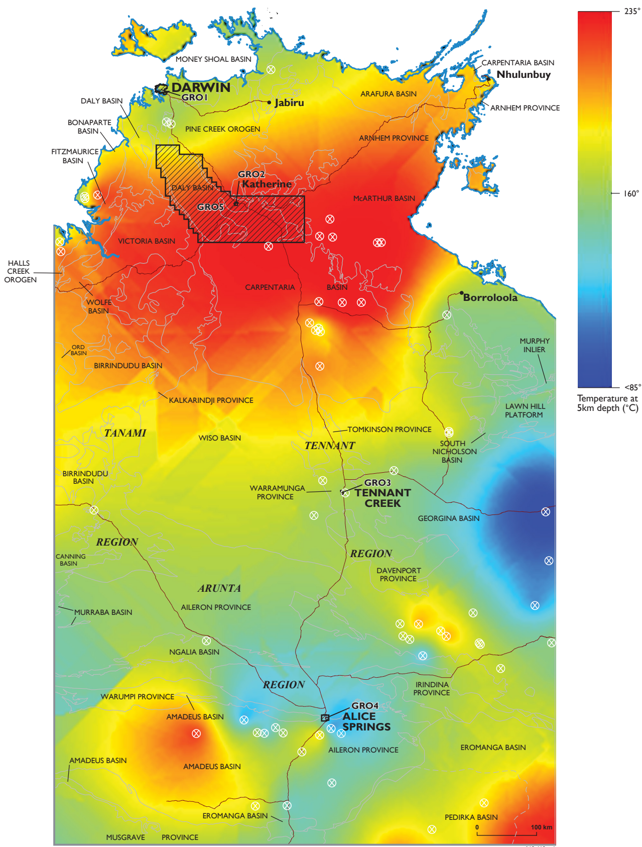
Geothermal image © Commonwealth of Australia (Geoscience Australia) 2010 A16-110c.ai
