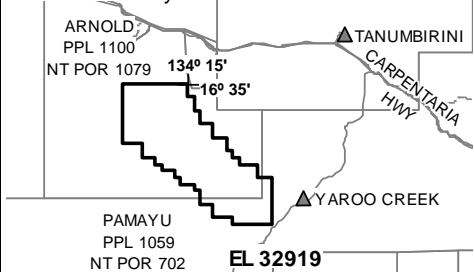
Not To Scale NMIG Map Sheet No: 5764
